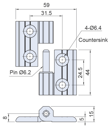
SPECIFICATIONS: Left Opening
