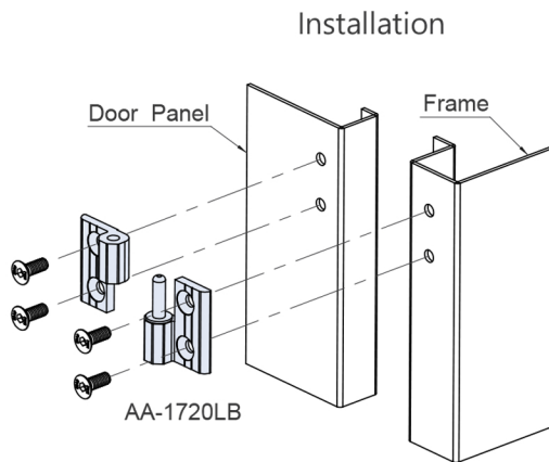
SPECIFICATIONS: Left Opening
