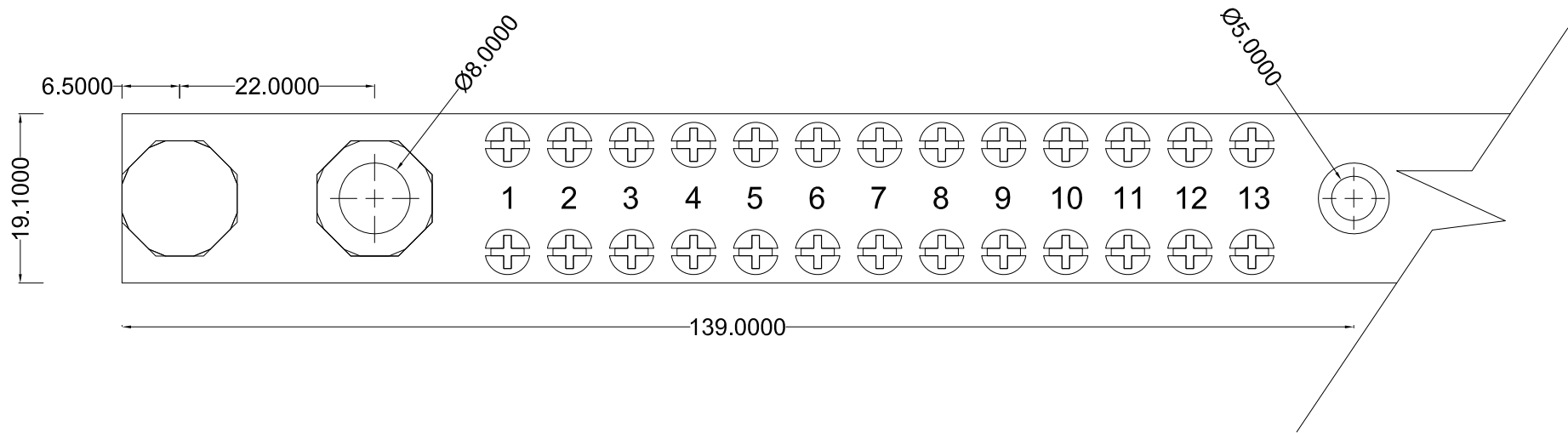
Typical EN6, 12 and 18 showing mounting holes
