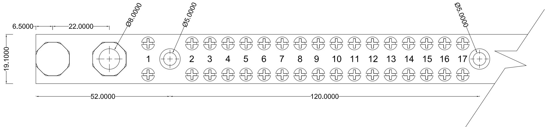
Typical EN24, 36 , 42 and 48 showing mounting holes
