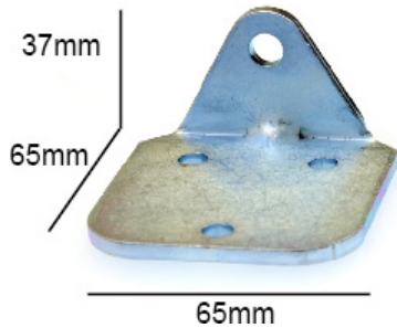
gskbracket4mm
