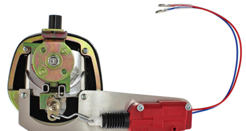
Rear Elevation in locked position
