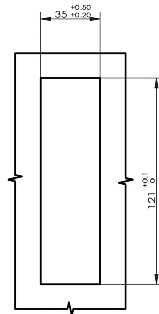
NSQBZ EURO BARREL & KEY (KEY BARREL SOLD SEPARATELY)
